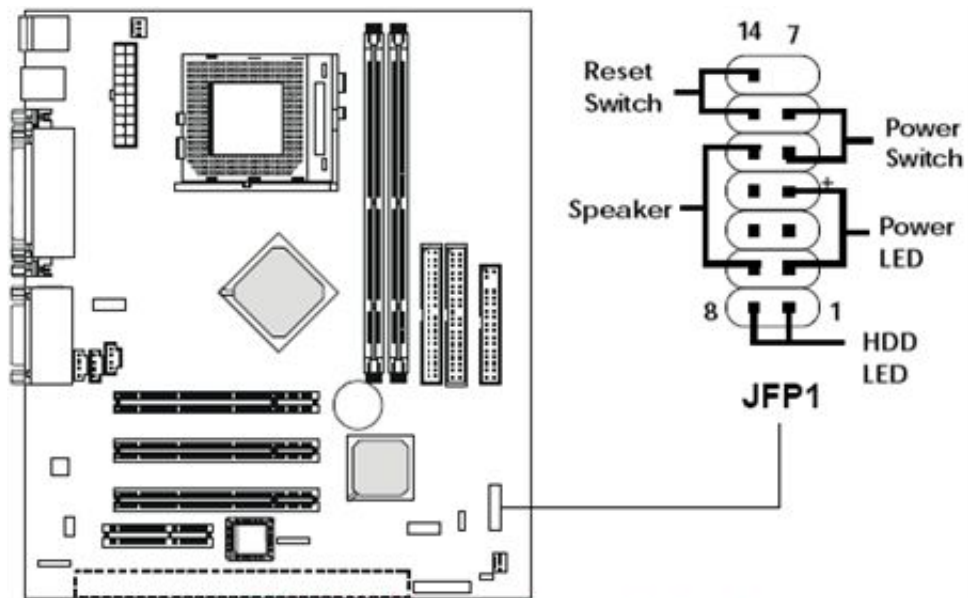
MSI MS-6368 front panel connection header
